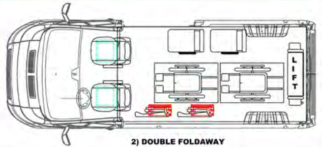
2) DOUBLE FOLDAWAY
